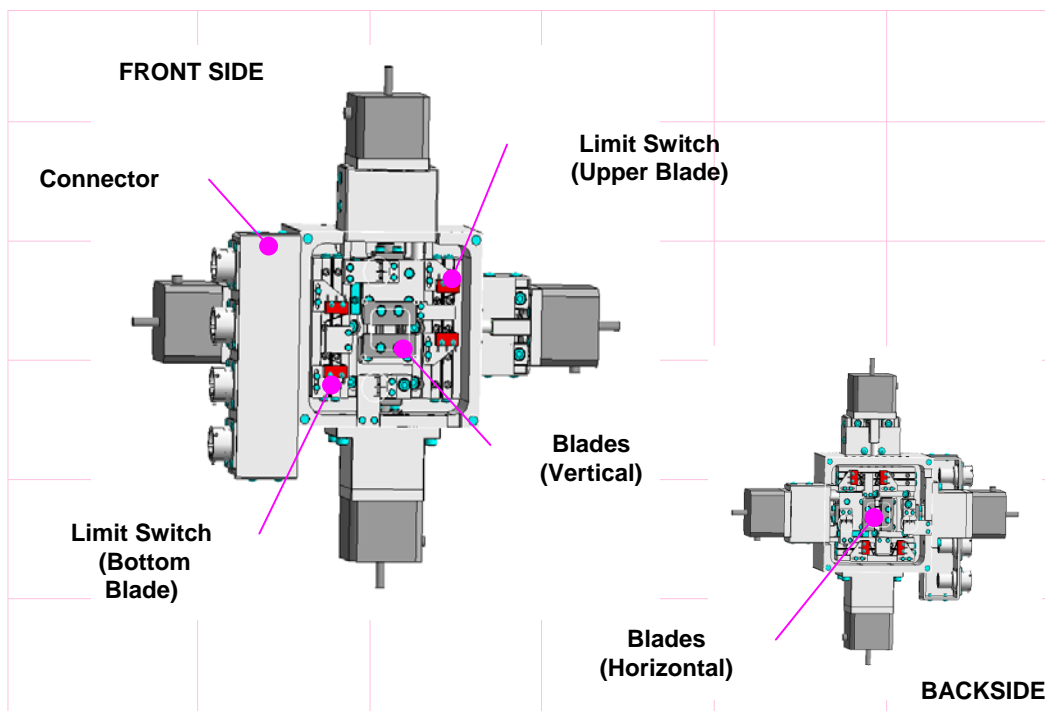
The slit is installed in a XAFS instrument.
